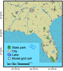
Fig. 3: Current distribution of urban and preserved areas in the Southeast US. The grid indicates the horizontal resolution at which the model performed (~20x~20 km)
